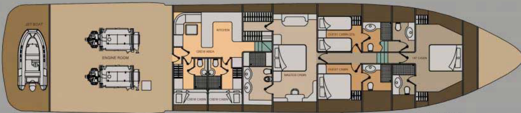
LOWER DECK
